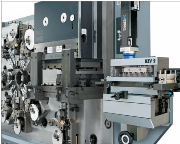
NC radial gripper feed unit RZV 2
