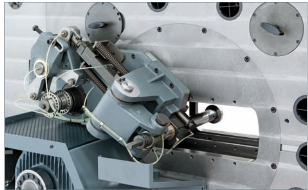
Central mandrel
